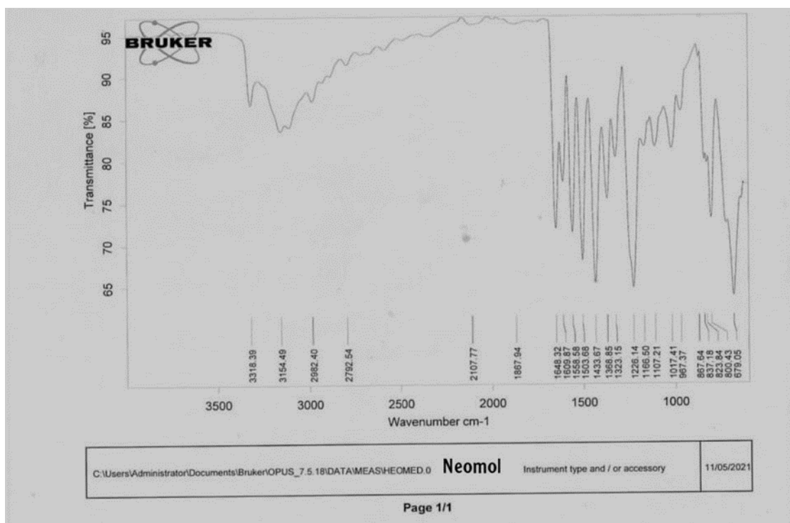
Figure S3: FT-IR Spectroscopy of Neomol(Neopharma®)
