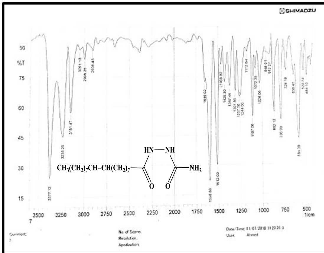
Figure S1: Infrared spectrum of [E 1 ]
