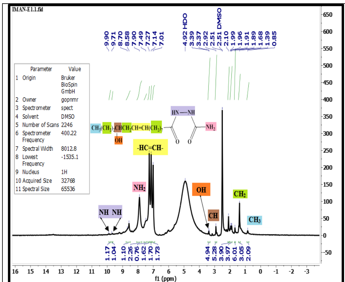
Figure S7: 1 H-NMR spectrum the compound [E 4 ]
