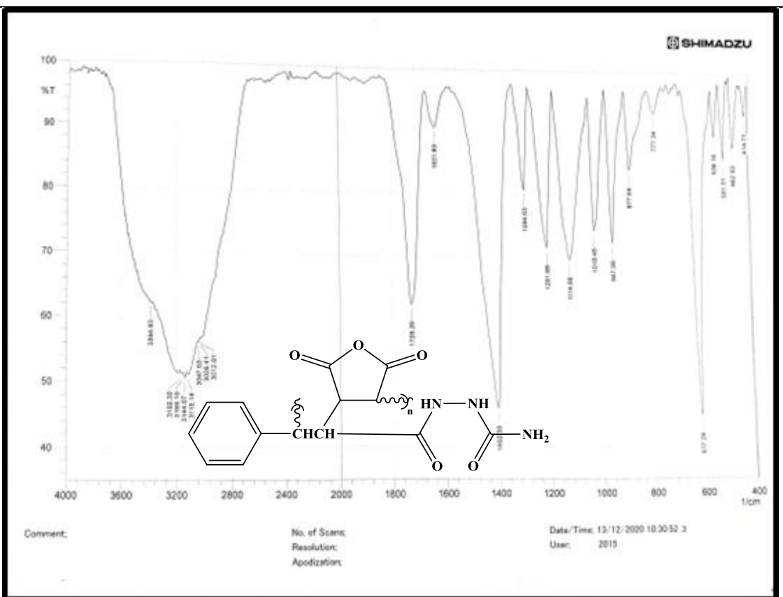
Figure S9: Infrared spectrum of [ Ep 5 ]
