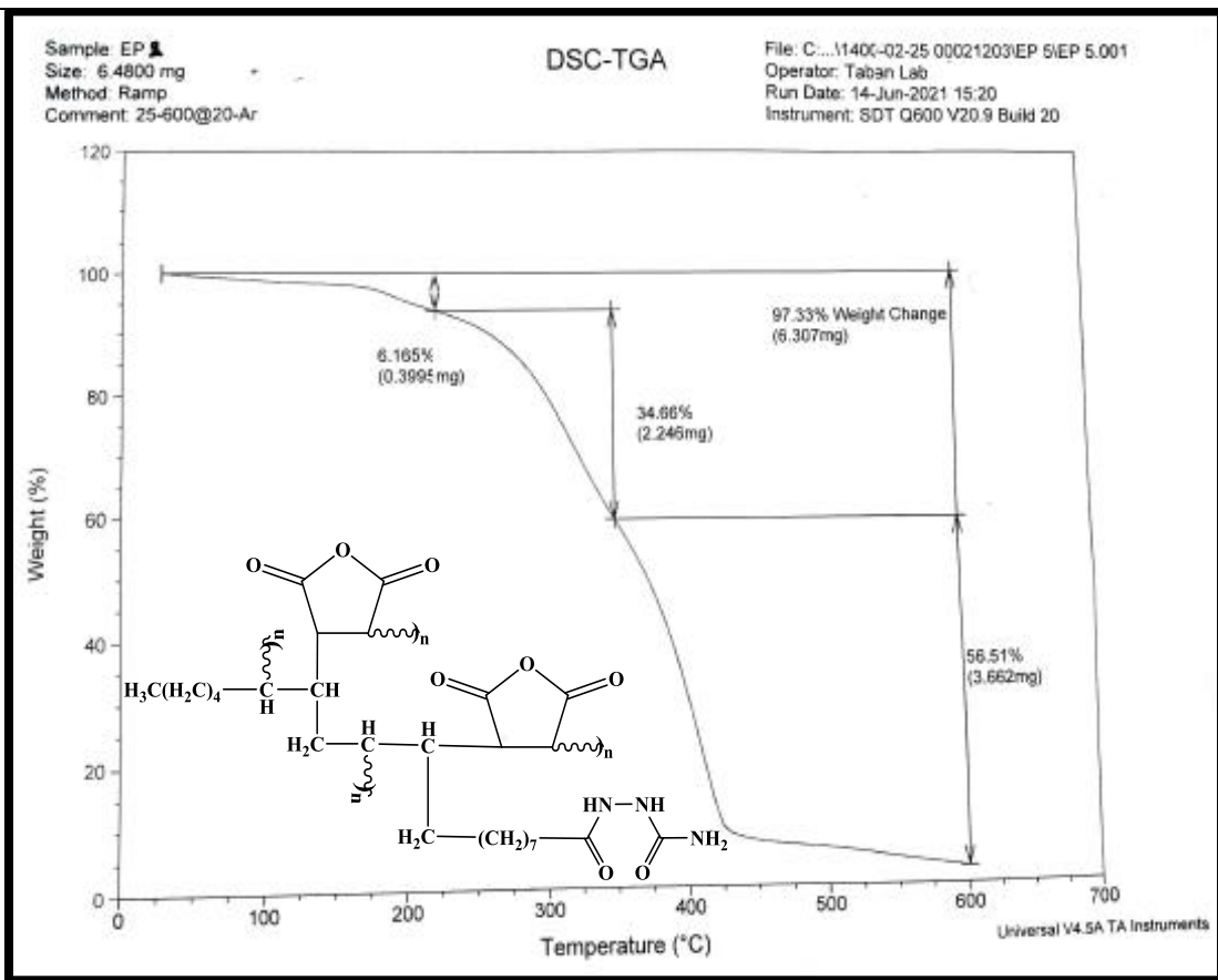
Figure S10: Thermogram analysis of CoPolymer Ep 2
