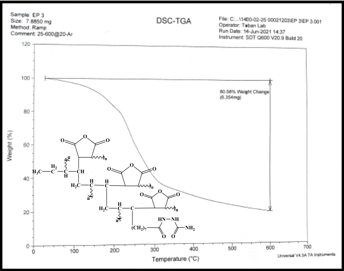
Figure S11: Thermogram analysis of CoPolymer Ep 3
