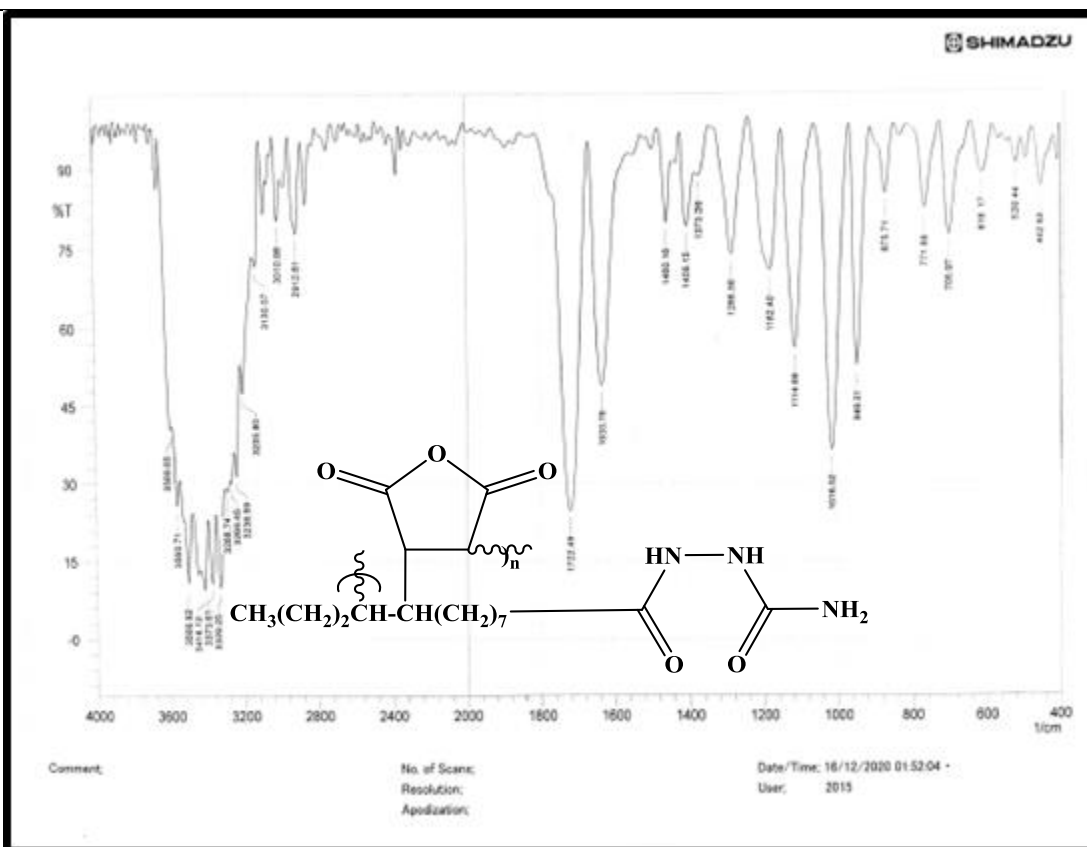
Figure S8: Infrared spectrum of [ Ep 1 ]
