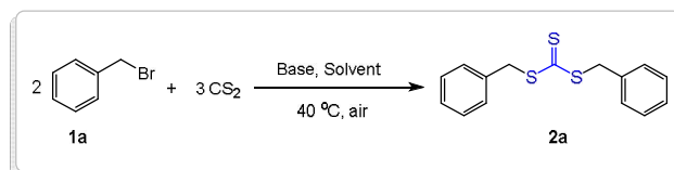
Scheme 1. Model reaction for the synthesis of the product 2a.
