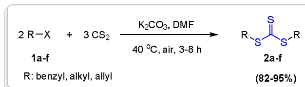
Scheme 2. Synthesis of the trithiocarbonates.
