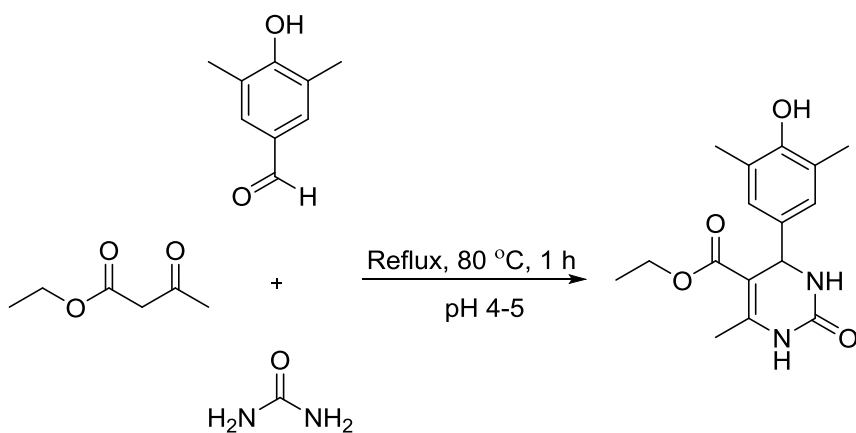
Scheme 3: synthesis of 3
