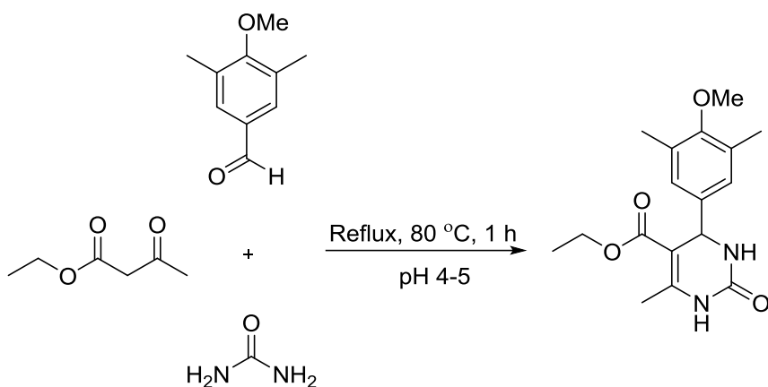
Scheme 1: synthesis of 1
