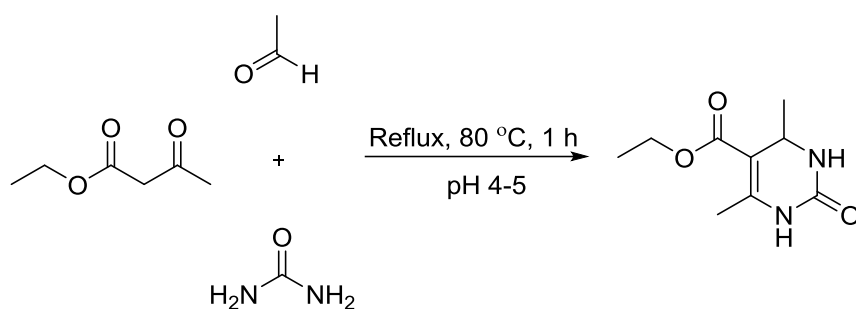
Scheme 4: synthesis of 4
